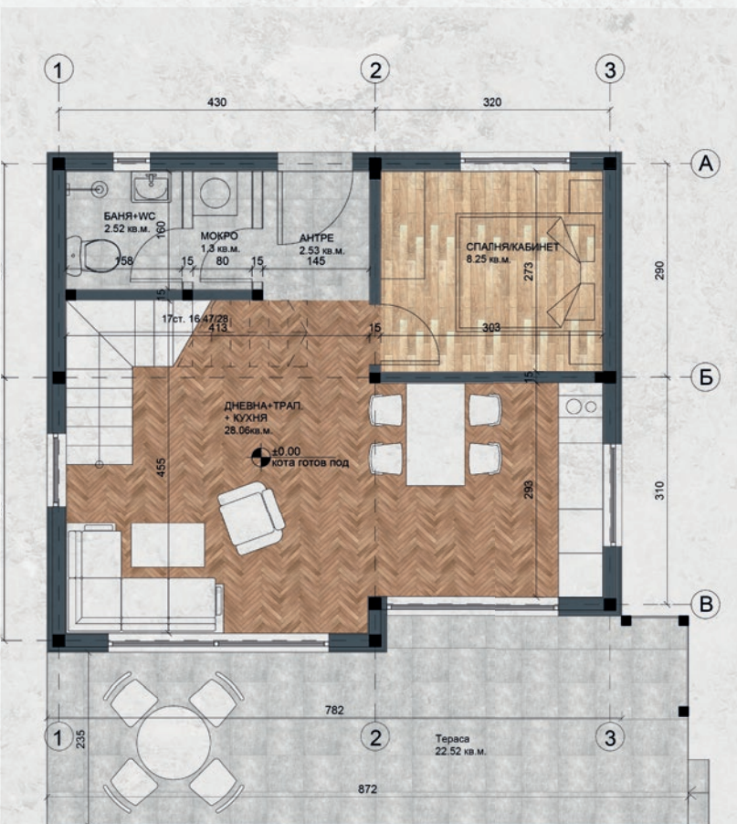
Plan M1:50 Area: 119.72 sq. m.
